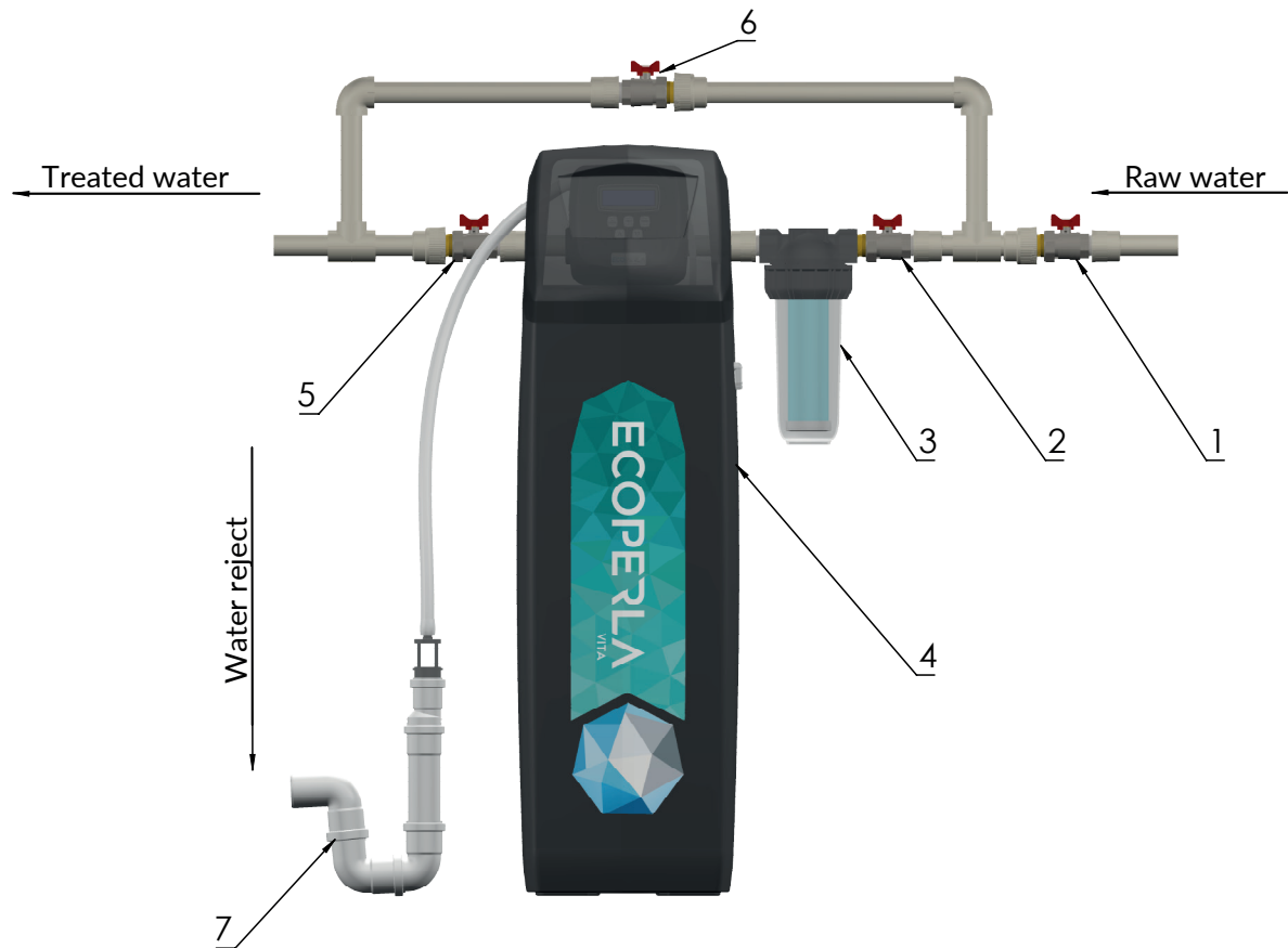
ECOPERLA VITA CONNECTION DIAGRAM
